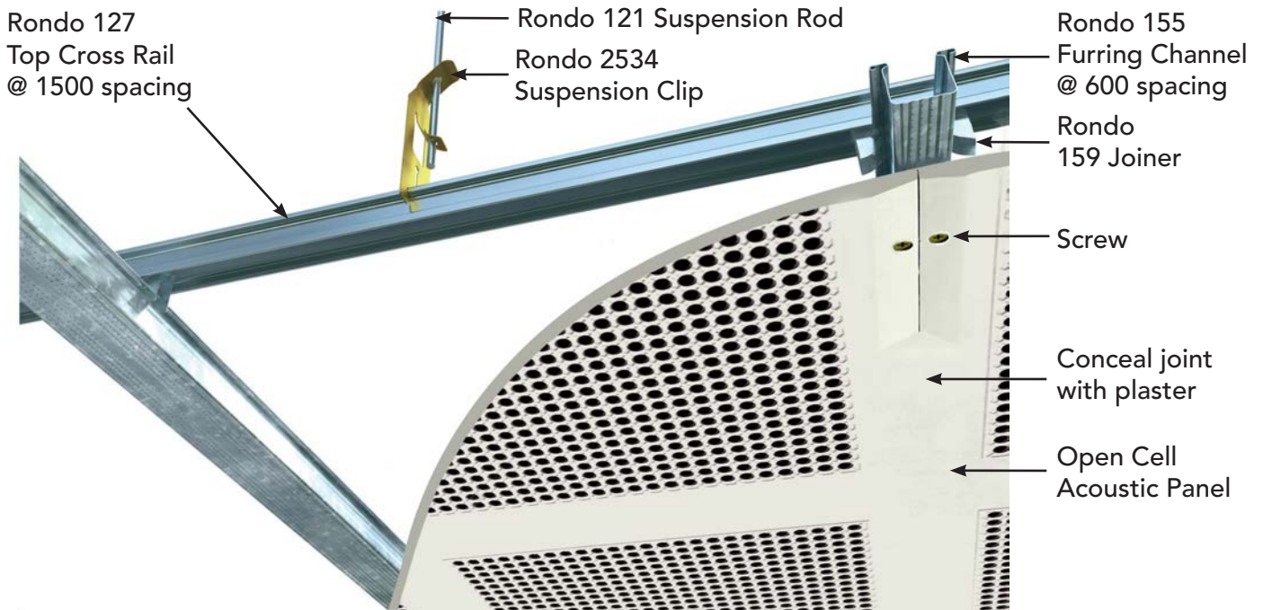
BOTTOM VIEW Typical Ceiling Installation with RONDO KEY-LOCK® Ceiling System
